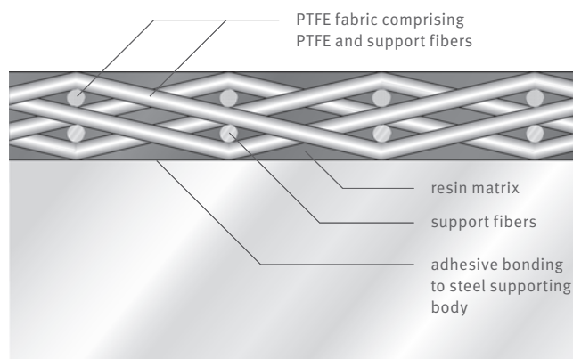
Structure of the ELGOGLIDE fabric
