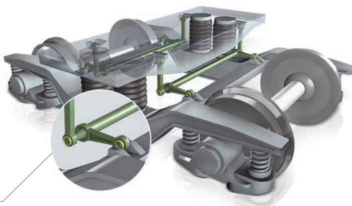
Maintenance-free radial spherical plain bearing for stabilizing railcar bodies and for the suspension of shock absorbers
